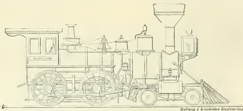
FAMOUS MORRILL ENGINE, BUILT BY VERMONT CENTRAL RAILROAD ABOUT 1863. From drawing loaned by E. R. Russell, Burlington, Vt.
